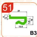
51 UHMW Plastic Strips
